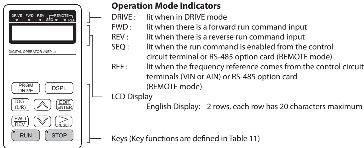
Fig 9-a LCD Digital operator component names and functions
