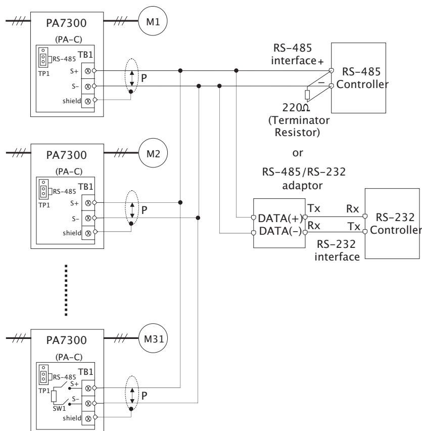
Fig. 15 Wiring for PA-C METASYS/MODBUS Protocol communication
