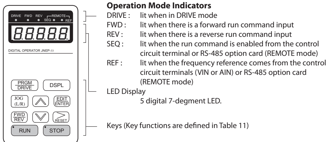
Fig 9-b LED Digital operator component names and functions
