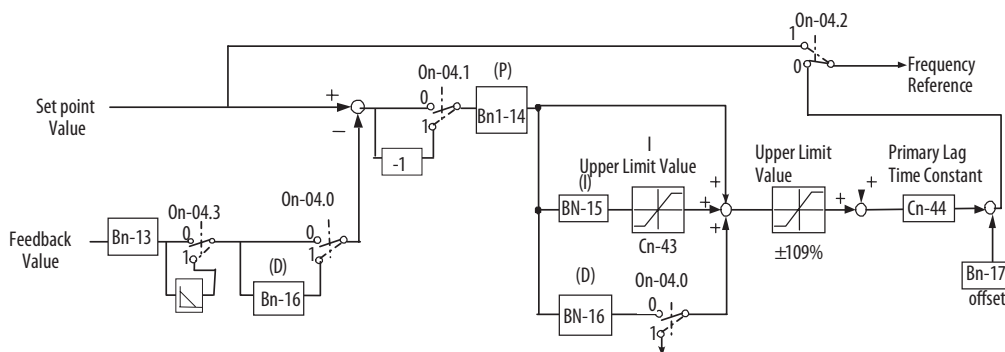
Fig 11-(b) Block Diagram of PID Control Section (For Versions xx and Later - Note 3))
