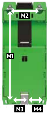
Mounting Dimensions
