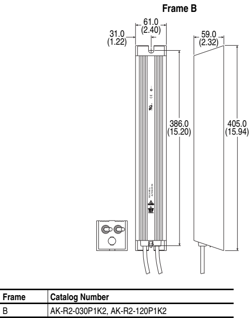
Figure B.2 Dynamic Brake Modules – Dimensions are in millimeters and (inches)
