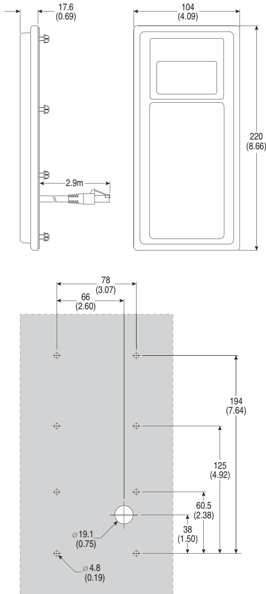
Figure B.8 Remote (Panel Mount) HIM – Dimensions are in millimeters and (inches)
