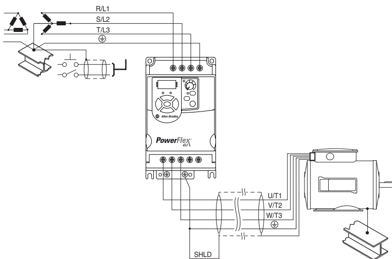
Figure 1.3 Typical Grounding
